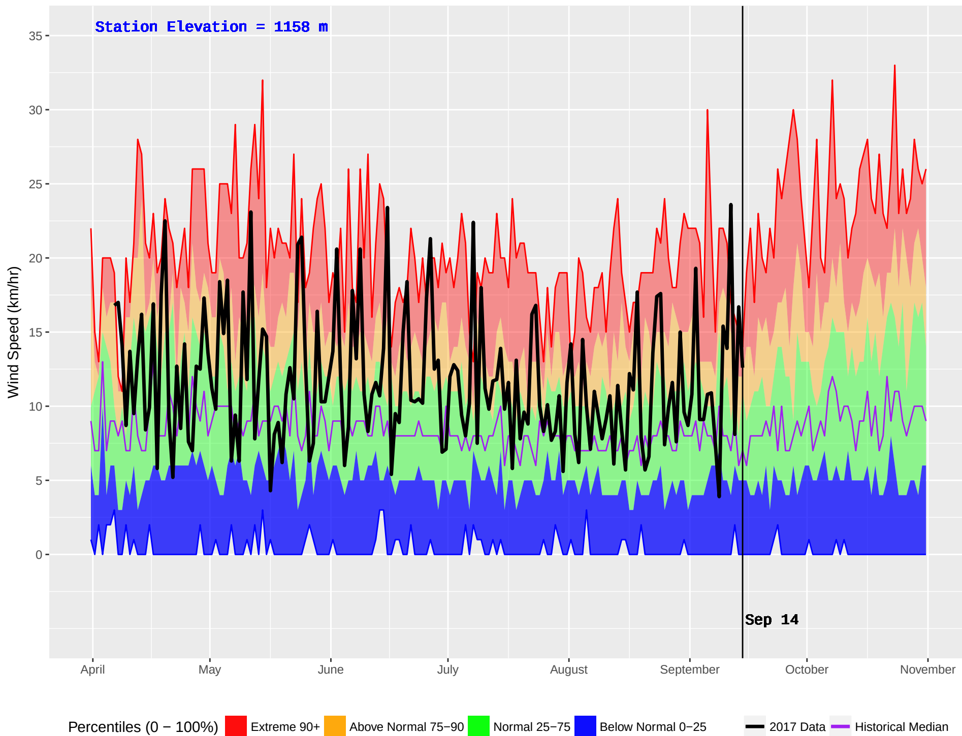
LONE BUTTE (218) : Historical (1987–2016) and Current (2017) Noon Wind Speed
