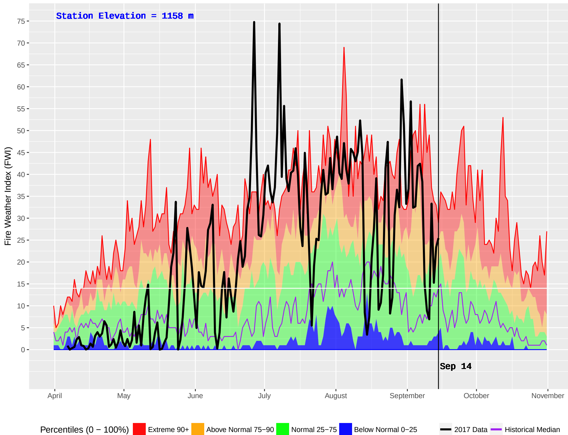
LONE BUTTE (218) : Historical (1987–2016) and Current (2017) Noon Fire Weather Index (FWI)
